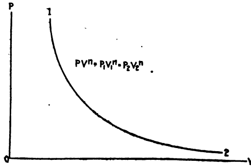
FIG. 6.—Exponential change of air.
